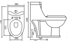
FLORA- 1015 L 720 W 380 H 690MM S TRAP - 225MM / P - TRAP
