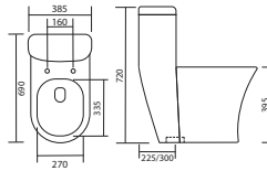
LIVION - 1001 L 690 W 395 H 720MM SIPHONIC - 225,300 MM
